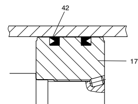
Lipseal Piston
