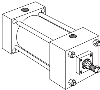
Style HB Cap Square (NFFPA Style ME4)
