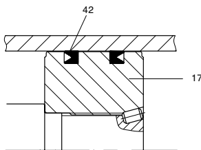
Lipseal Piston
