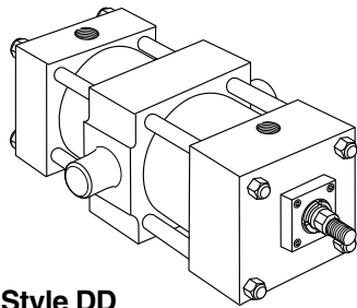
Style DD Intermediate Fixed Trunnion (NFPA Style MT4)
